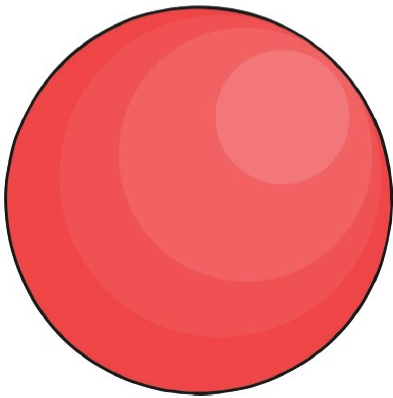
Sphere
