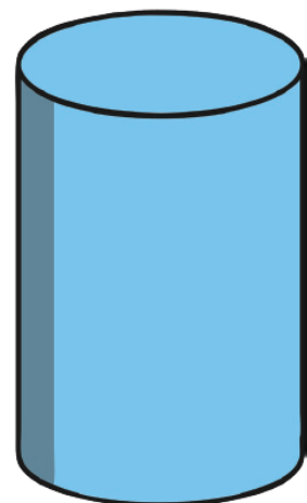
Cylinder
