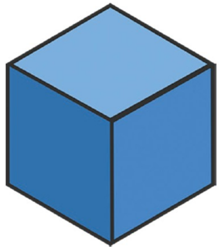
Cuboid
